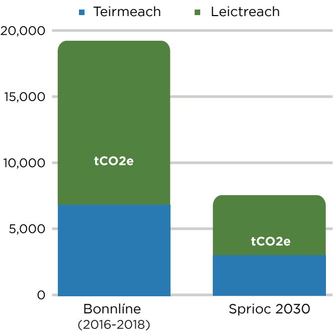
Fig 4. Spriocanna laghdaithe carbóin raon 1 & 2 go 2030
