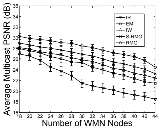
Fig. 10. The average PSNR performance when the WMN size in Fig. 6 increases from 18 to 44.
