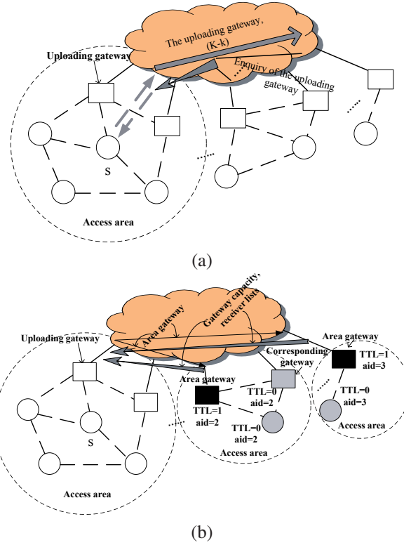
Fig. 4. An example of constructing a two-tier integrated architecture . Square nodes represent gateways. Circle nodes represent mesh routers/mesh clients. Black nodes and grey nodes are the senders and the receivers of AREA.CONSTRUCTION respectively.
