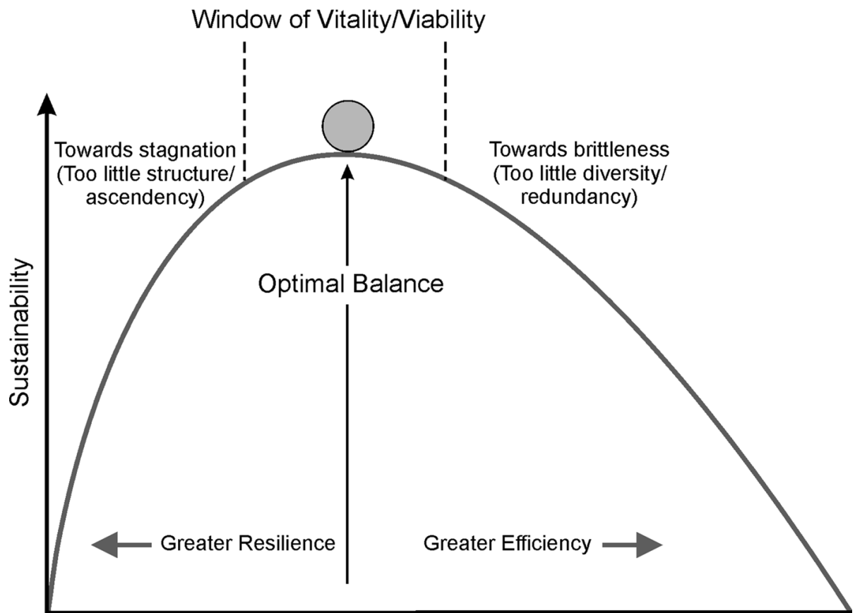
FIGURE 3.1 A model of sustainability as contingent balance between agonistic tendencies of overhead/resilience/uncertainty and ascendancy/efficiency/control, after Ulanowicz, et al. (2009) and Goerner, Ulanowicz and Lietaer (2009)
