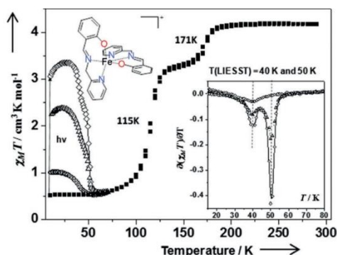
Figure: X_m T versus T iron(III) complex showing the LIESST effect at 10 K. Thermal relaxation after ( \circ ) irradiation at 647.1nm during 2 h, irradiation at 830 nm during 3 h ( \Delta ) and 12 h ( \diamond ). Structure of the complex cation is shown above the plot. The first derivative in the insert shows a double step relaxation curve. Transition temperatures are indicated.
