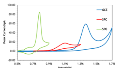
Figure 1: Cyclic voltammograms recorded at Nafion-modified glassy carbon (blue), screen printed carbon (red) and screen printed gold (green) electrodes in 0.1 M Phosphoric Acid containing 300 \mu M caffeine.
