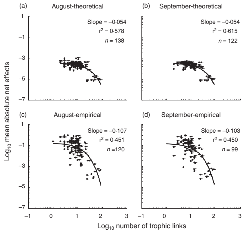
Fig. 3. Mean absolute net effect ( \pm SE) of each species on all other species in the mesocosm food webs plotted against number of trophic links (considering both predator and prey links for each species). Net effects were calculated (a, b) theoretically, using allometric predator–prey relationships and (c, d) experimentally, in the presence/absence of predators/competitors for the two experimental time periods. Values are plotted on a log-log scale with an exponential line of best fit.
