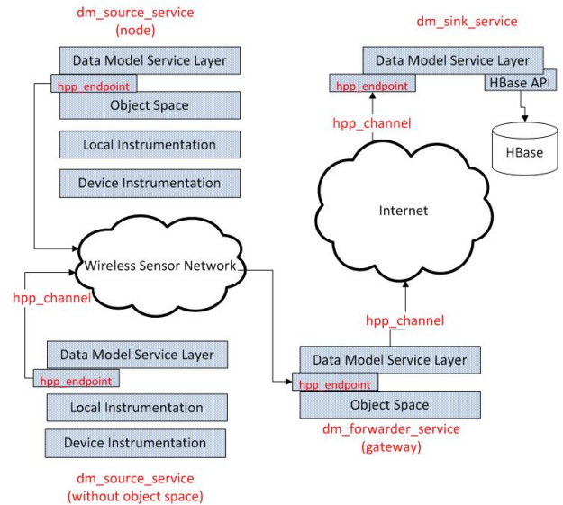
Fig. 1. Holistic Architecture
