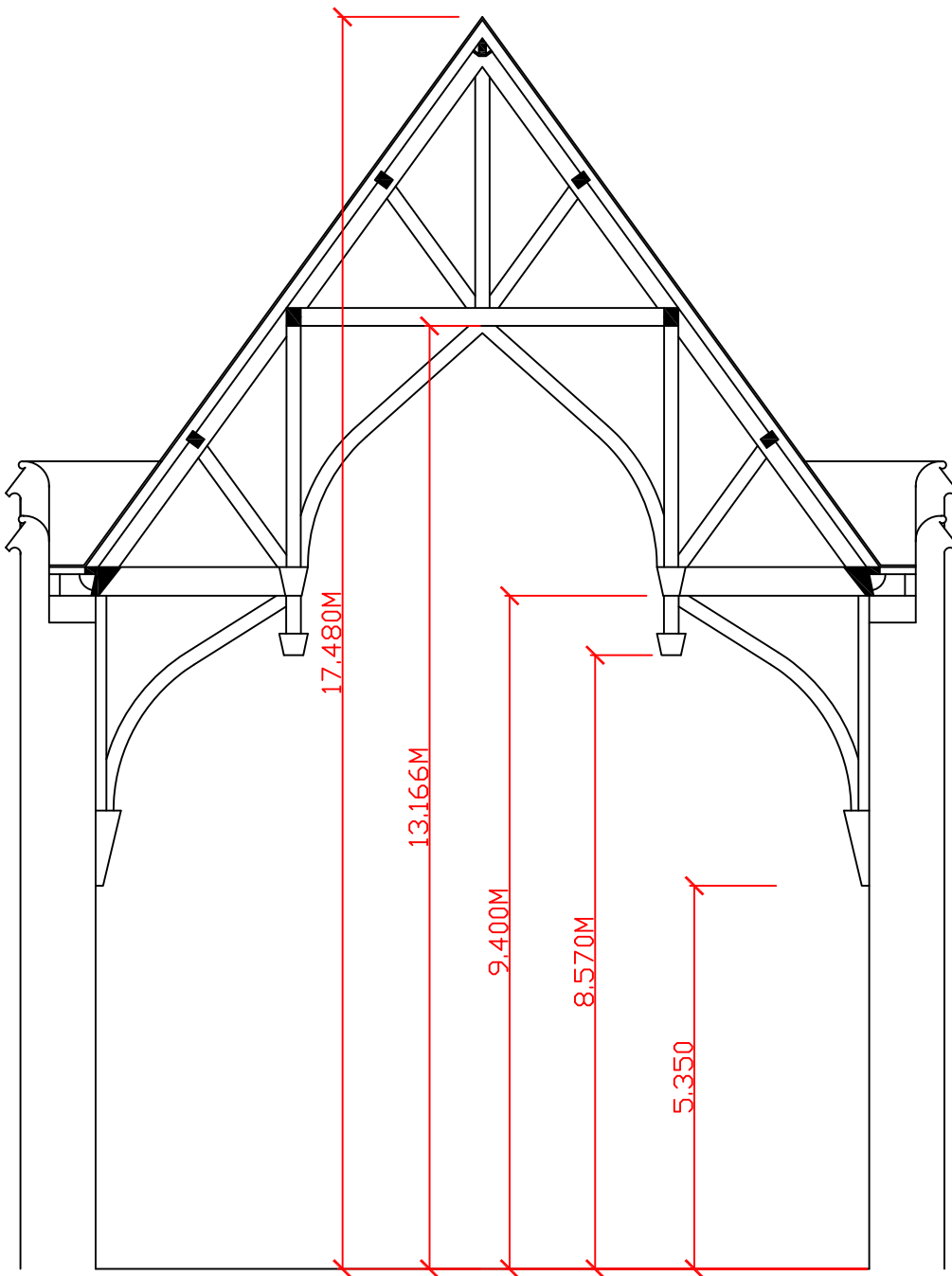
Typical Roof-section for Aula Maxima. (all dimensions are approx & should be checked on-site)
